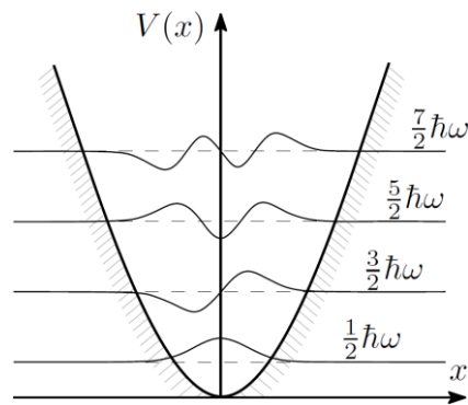
Fig. 1. First four wavefunctions of quantum harmonic oscillator.
